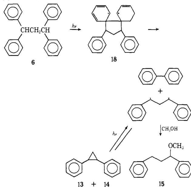
Scheme I. Mechanism for Photoreaction of 1,1,3,3-Tetraphenylpropane ( 6 )
